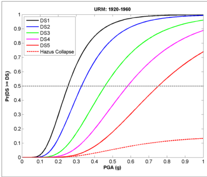
Fragility Curve
